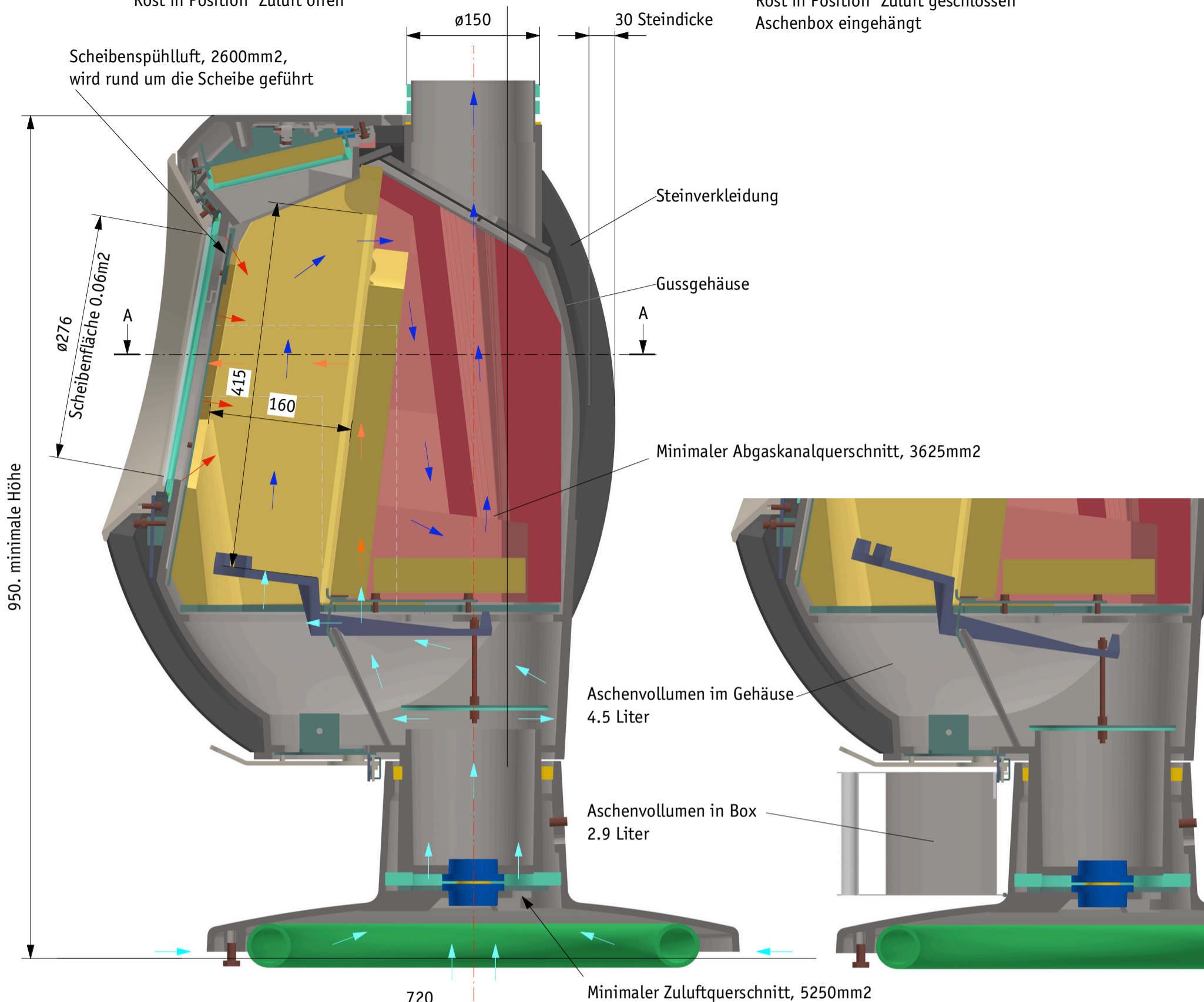
Totalschnitt Rost in Position "Zuluft offen"
